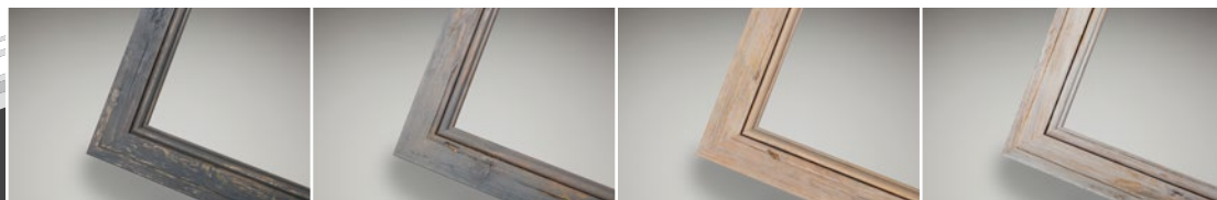
Basalt
